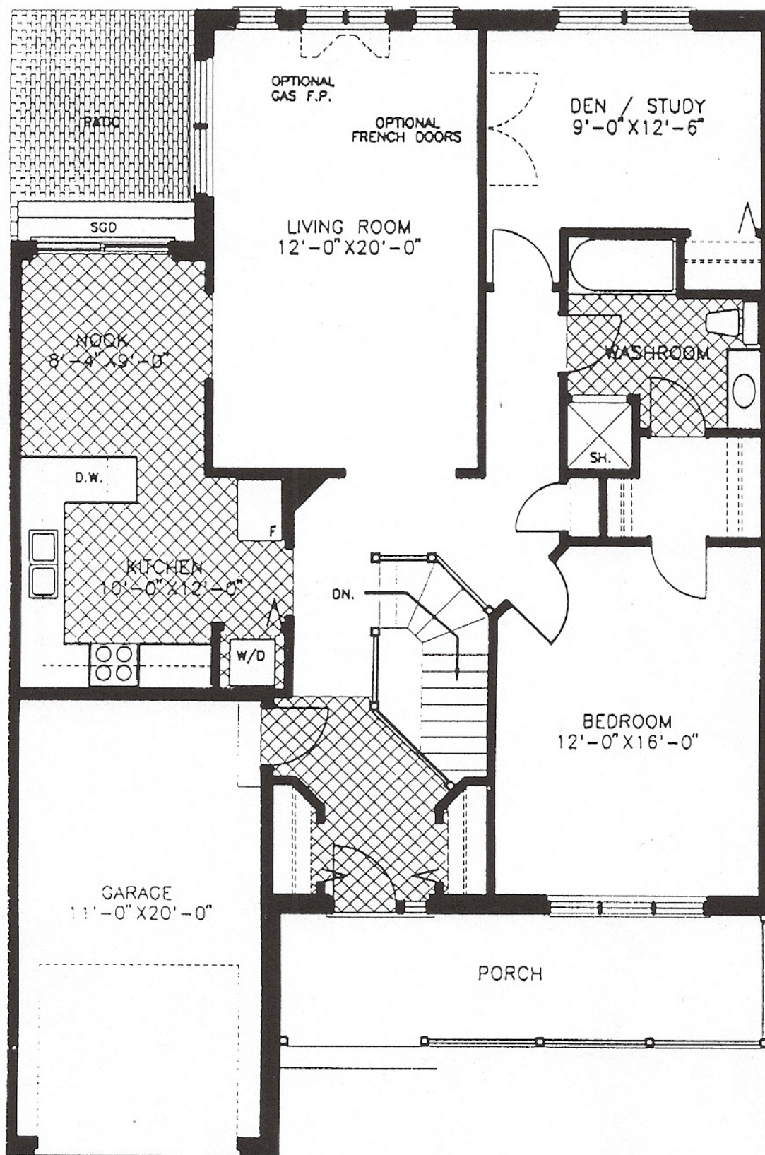
PEARL 1217 SQ FT DIMENSIONS SHOWN ARE APPROXIMATE AND MAY VARY
